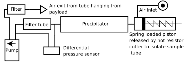
Figure 5: Flow diagram of the air sampling system.
