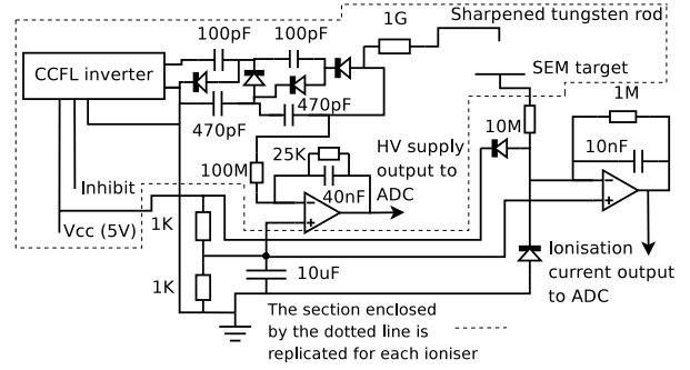
Figure 7: Circuit diagram of the electrostatic precipitator electronics.
