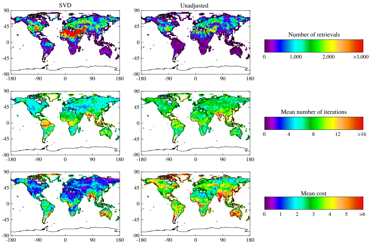
Fig. 10. Monthly mean retrieval statistics for the SVD (left) and unadjusted surface (right) runs on a 2.5° grid. From top to bottom, the maps show the total number of successful retrievals, the mean number of iterations needed before convergence, and the mean cost of successful retrievals.
