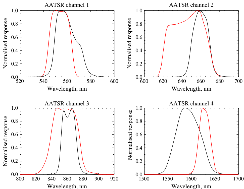
Fig. 1. AATSR (black) and MODIS (red) normalised visible channel response functions. MODIS channels closest to corresponding AATSR channels are shown.
