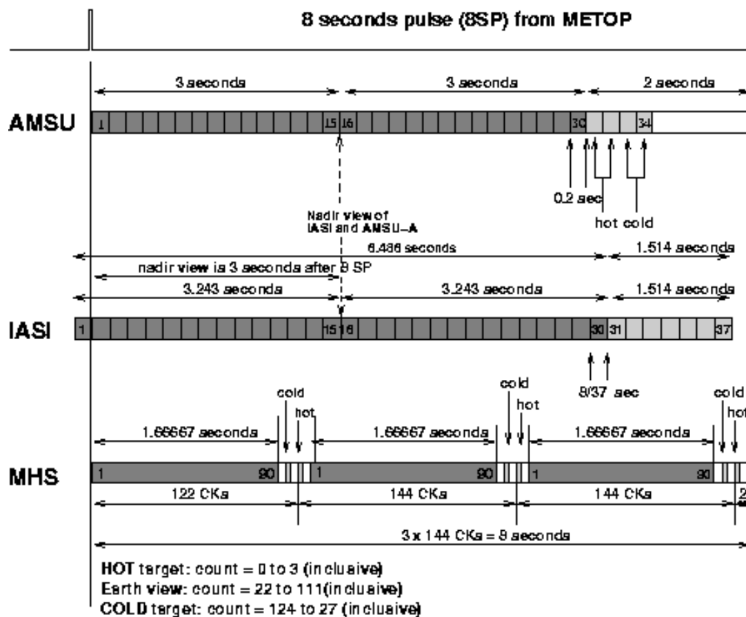
Figure 1: Synchronisation of IASI and ATOVS instruments on Metop
