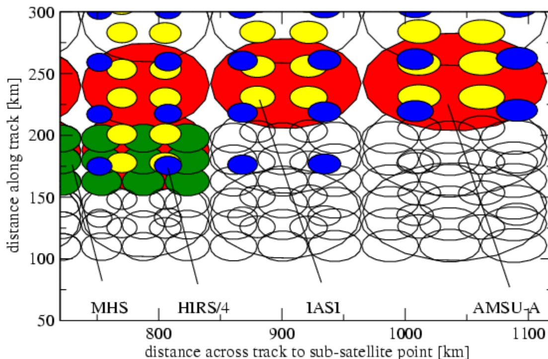
Figure 4: The collocation between IASI (yellow), AMSU (red), MHS (green) and HIRS (blue) is shown for four scan lines at the end of the IASI scan line. The distance along and across track is given in km.
