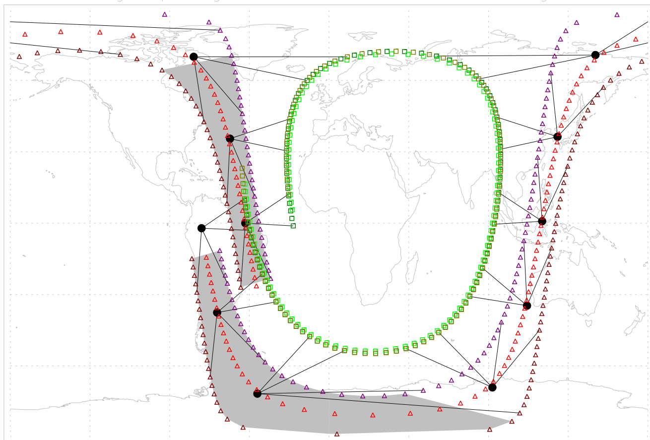
Tangent point geolocation for max, min azimuth angles
