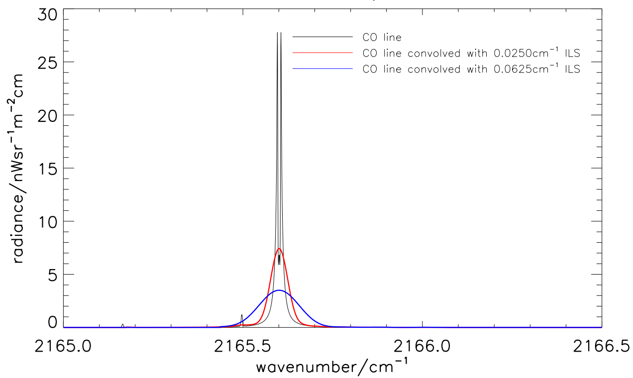
CO line convolved with 0.0250\text{cm}^{-1} and 0.0625\text{cm}^{-1} instrument line shapes at 30km
