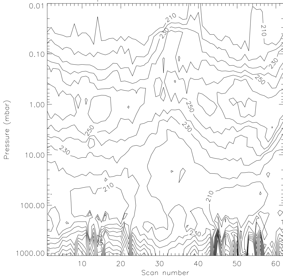
Temperature retrievals from Orbit 504
