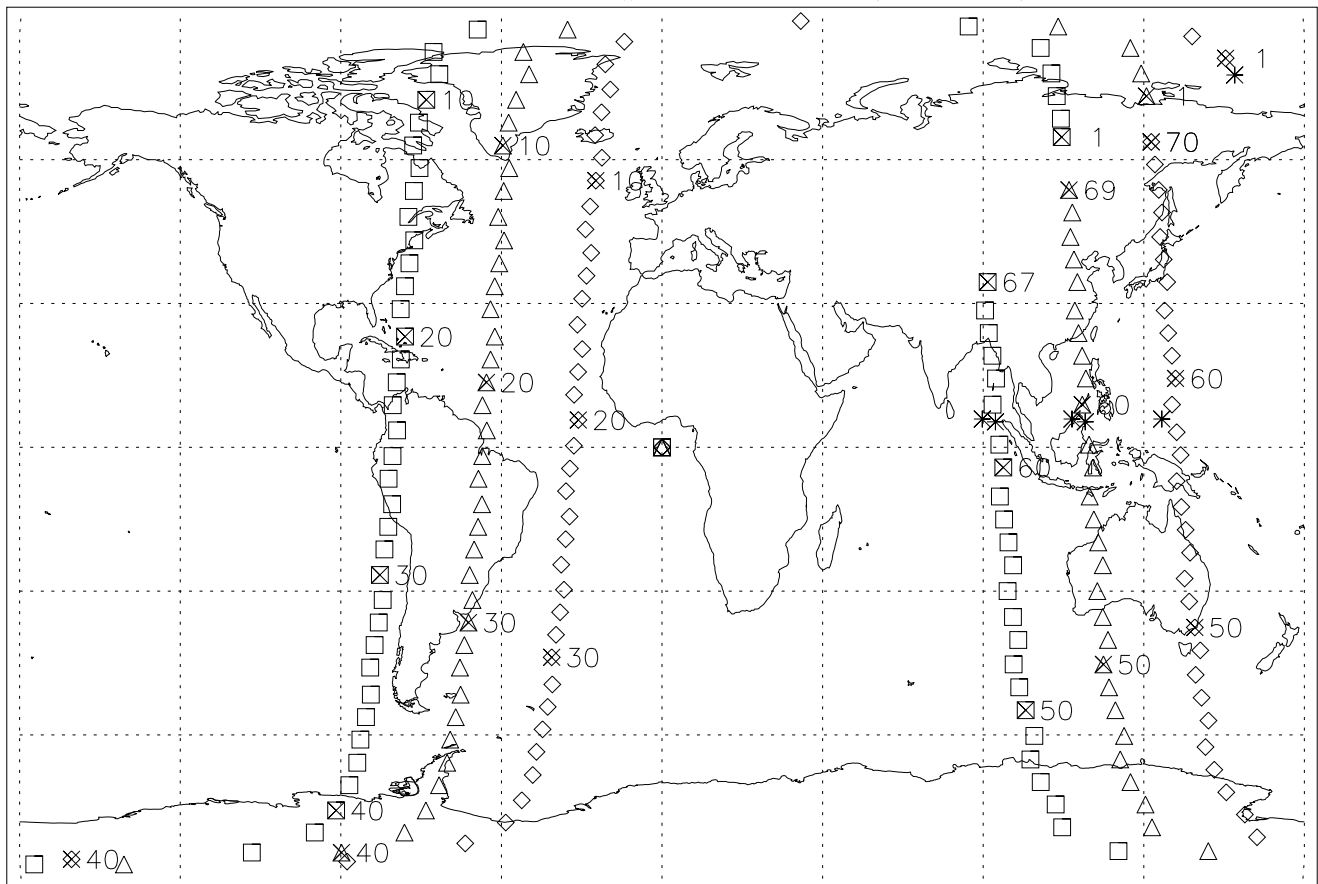
MIPAS Scans: Orbit#2081–2083 (24Jul02)
