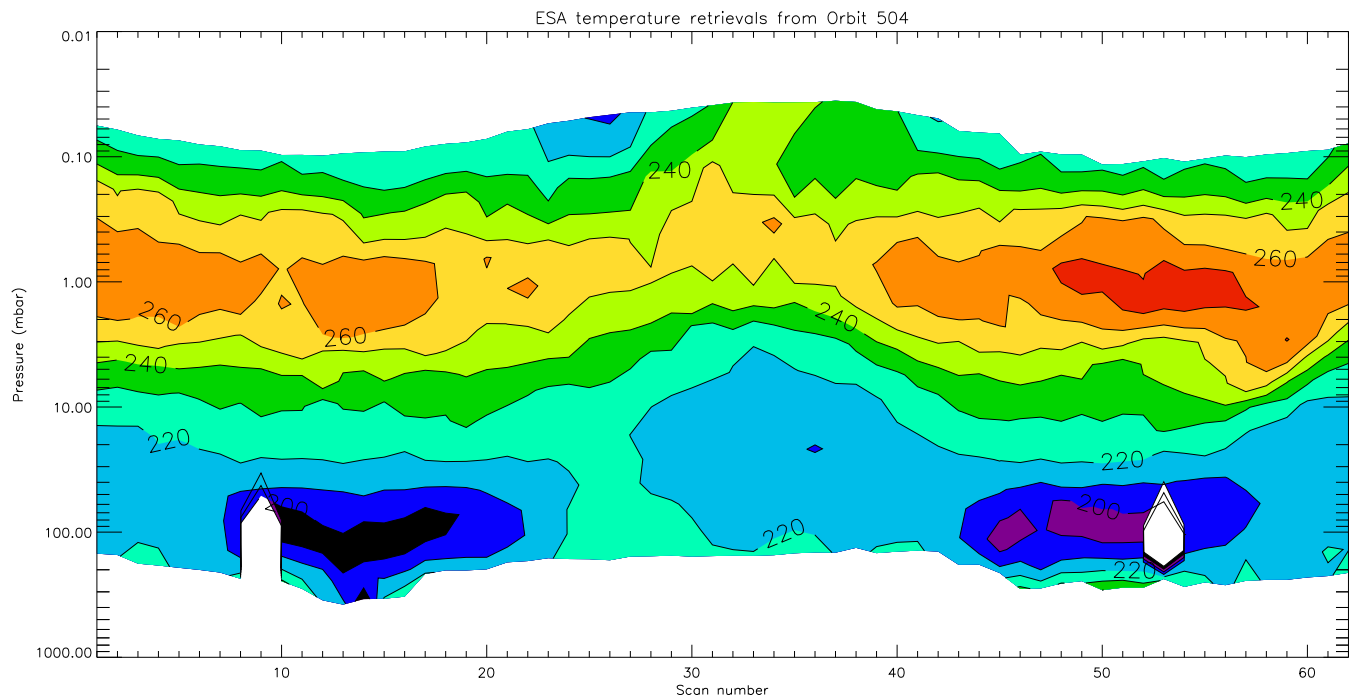
OPTIMO - ESA temperature at nominal altitudes
