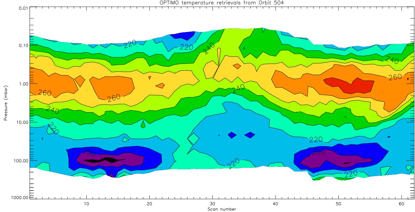
ESA temperature retrievals from Orbit 504
