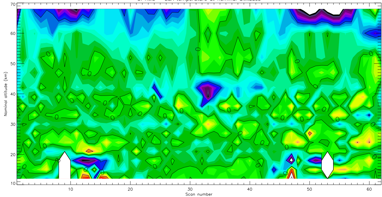
OPTIMO - ESA temperature at nominal altitudes
