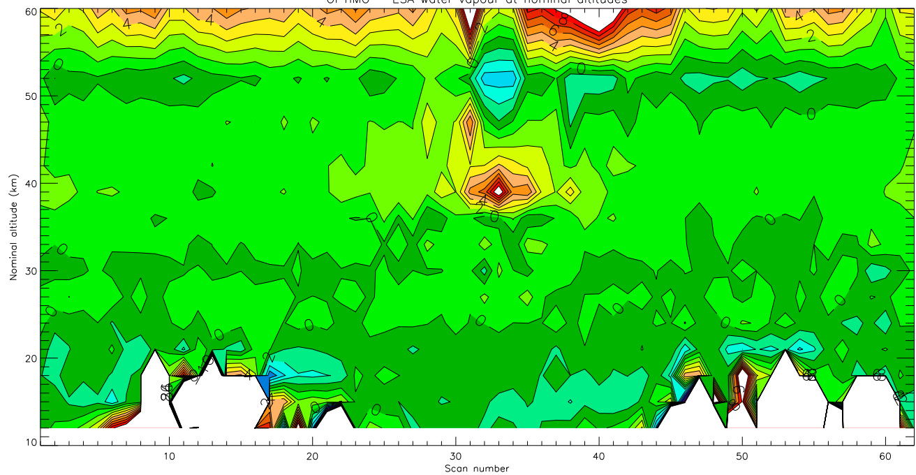
OPTIMO - ESA water vapour at nominal altitudes
