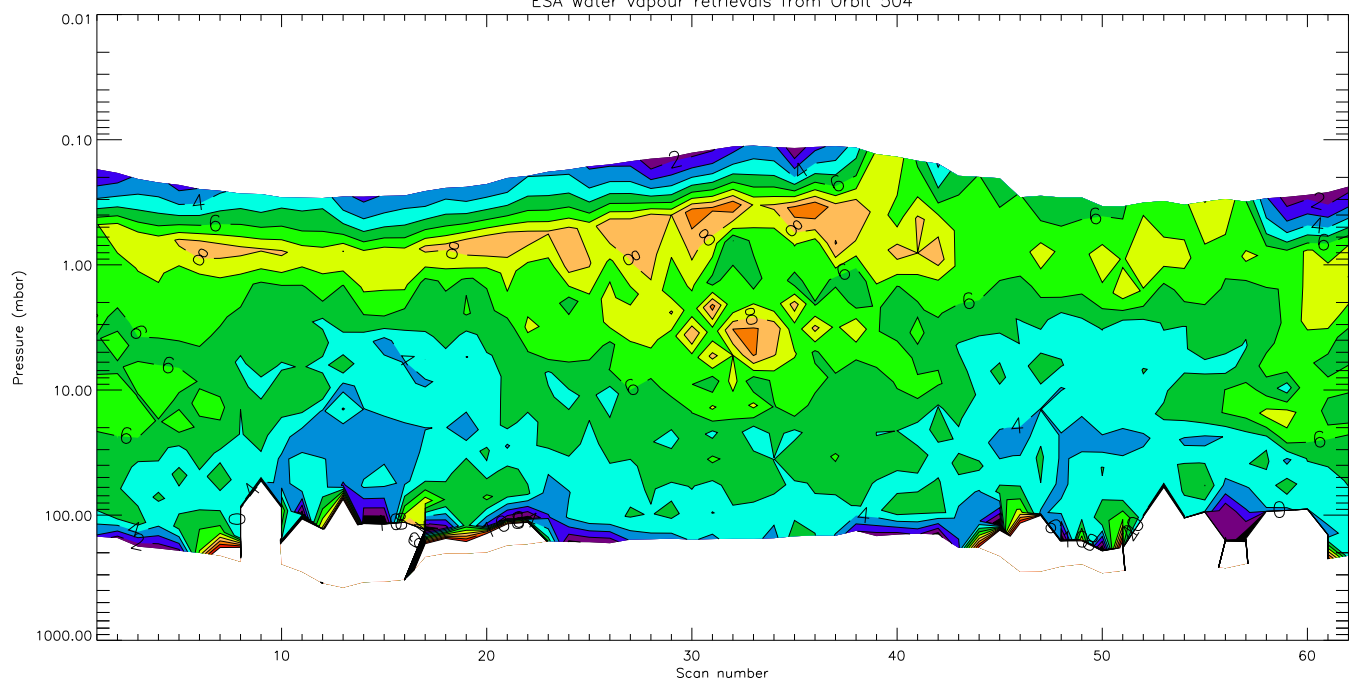
OPTIMO - ESA water vapour at nominal altitudes
