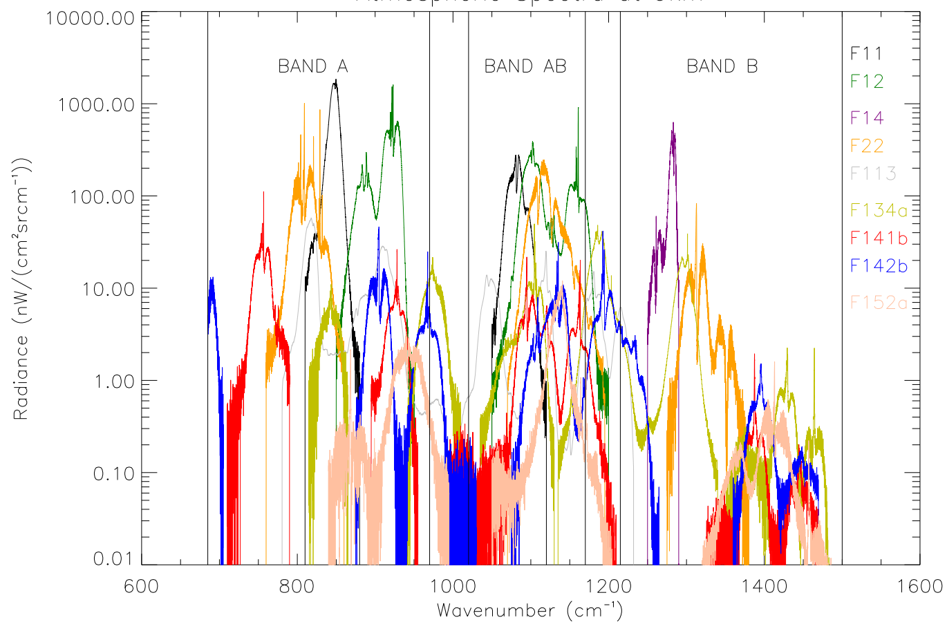
Atmospheric Spectra at 9km
