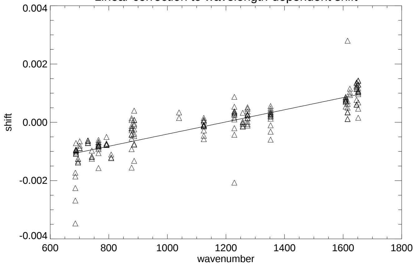
Linear correction to wavelength-dependent shift
