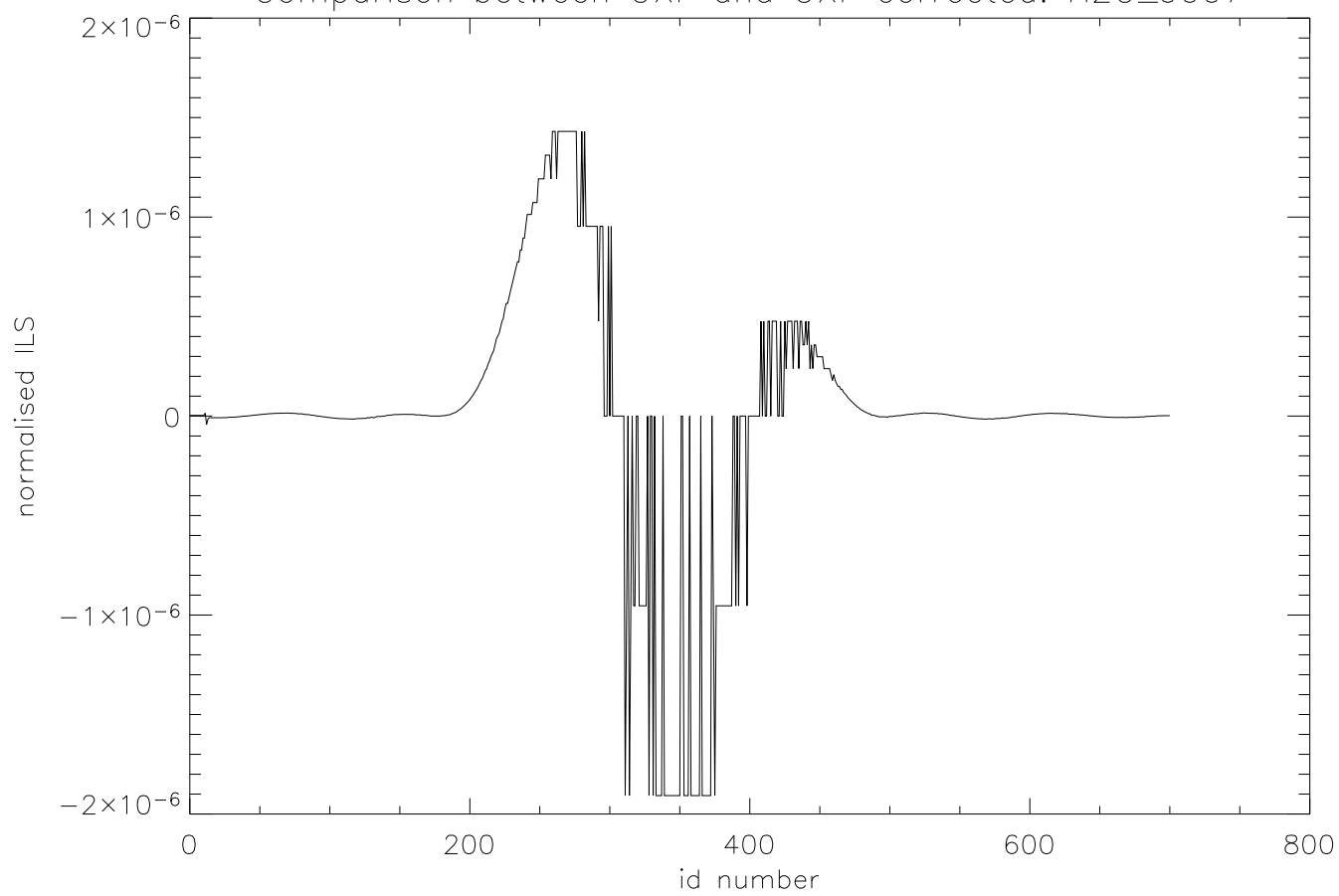
Comparison between OXF and OXF corrected: H2O_0007
