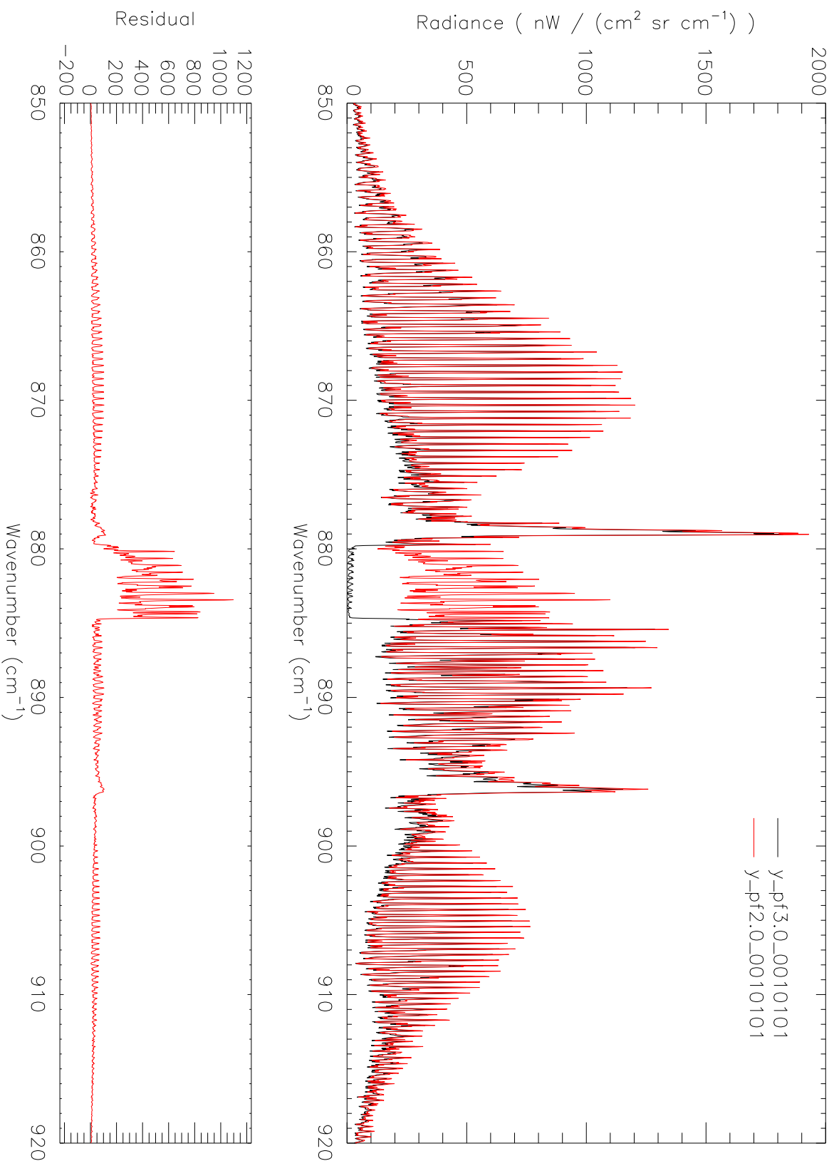
HNO 3 model spectra, 20 km tgh, HITRAN–MIPAS–PF3.0 and HITRAN–MIPAS–PF2.0
