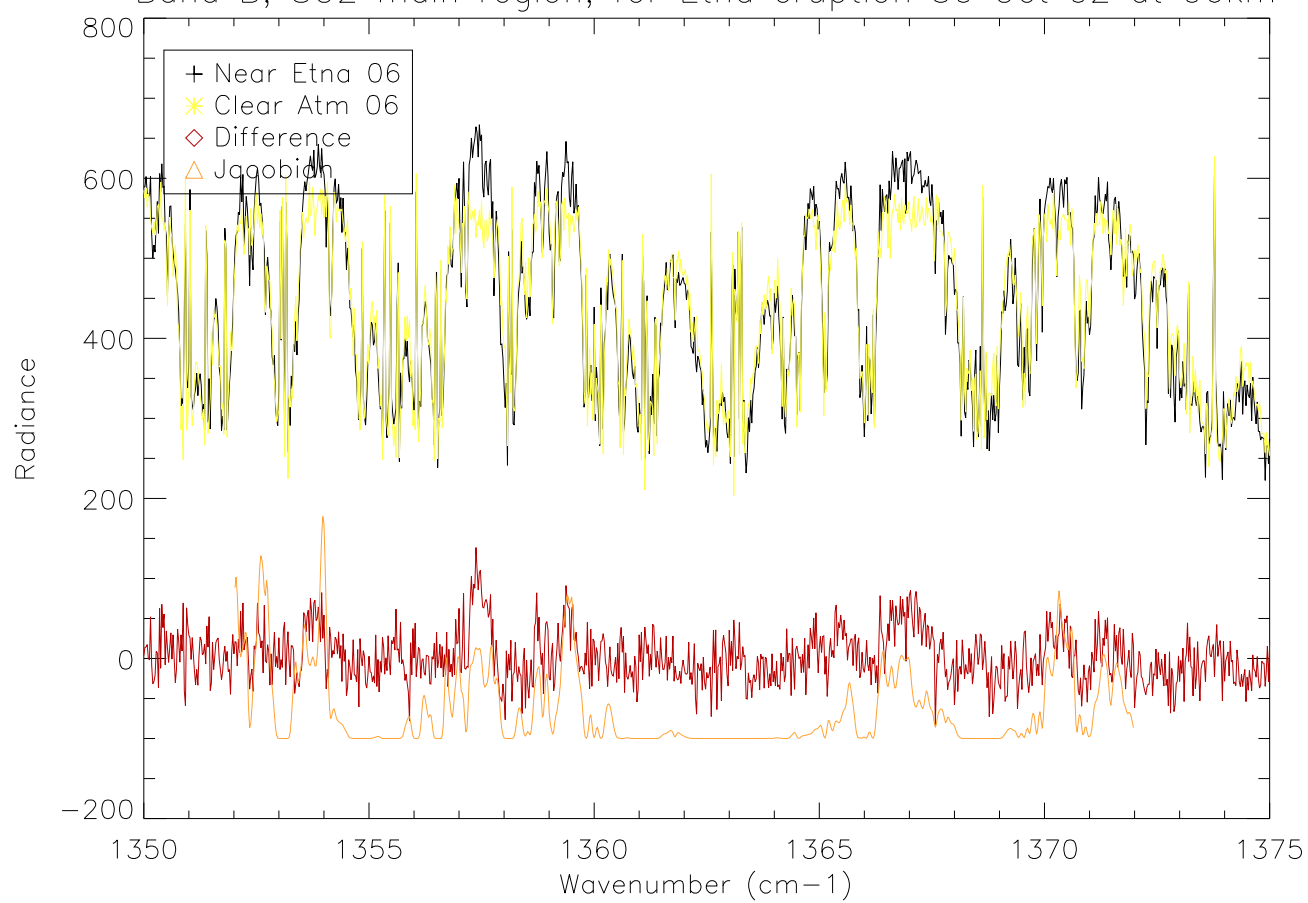
Band B, SO 2 main region, for Etna eruption 30 Oct 02 at 06km
