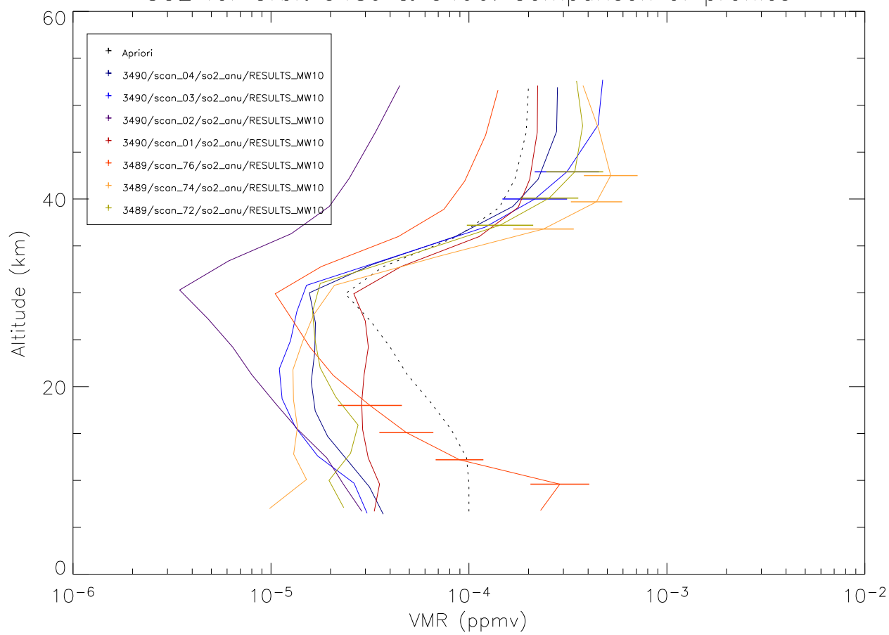
SO2 for Orbit 3489 & 3490. Comparison of profiles
