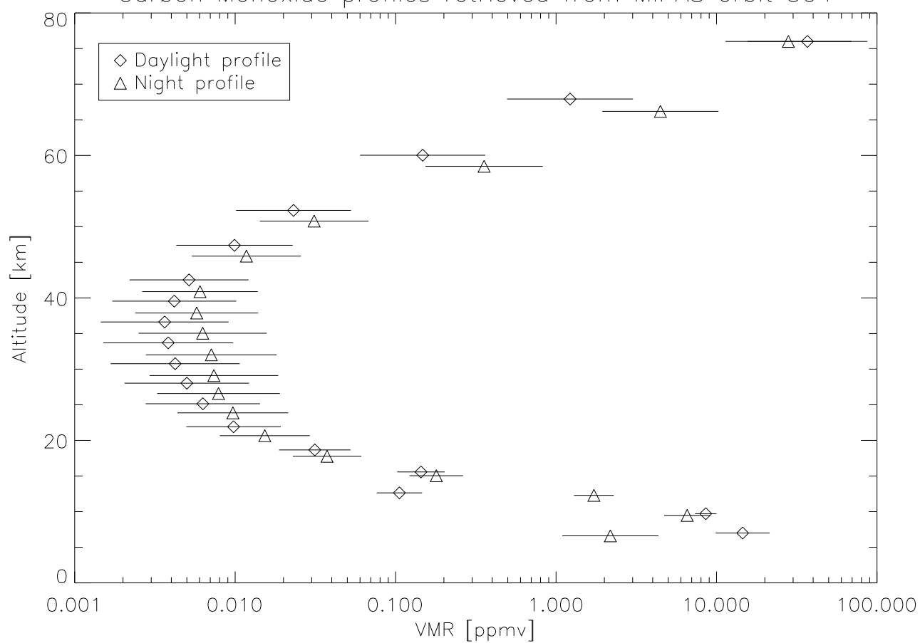
Carbon Monoxide profiles retrieved from MIPAS orbit 504
