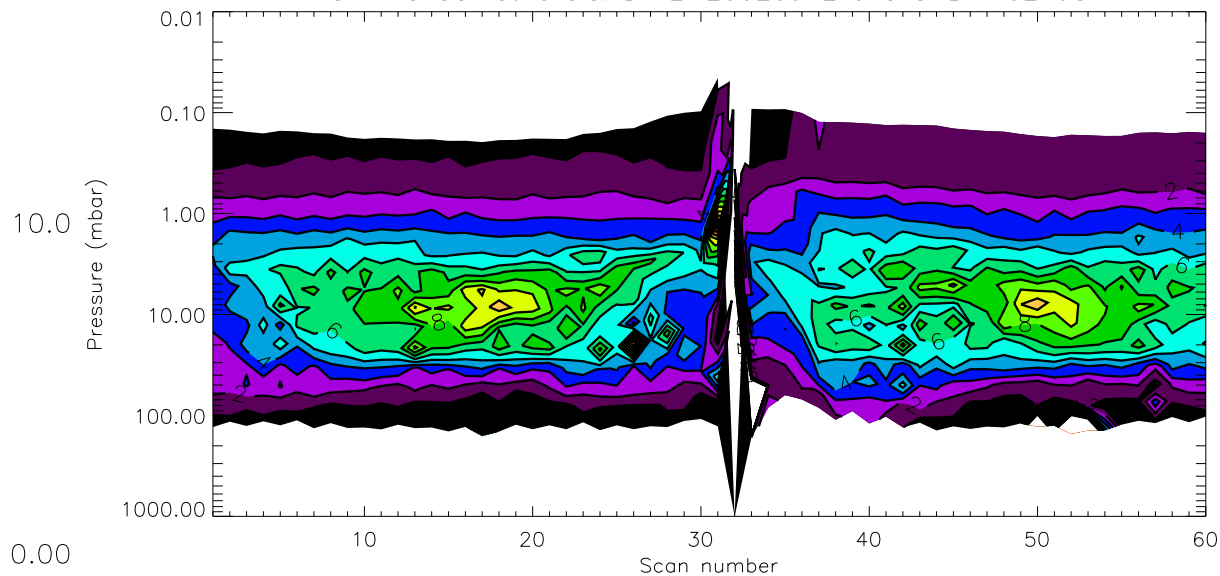
OPTIMO O3 retrievals: DATE=20020912 and ORBIT=02798
