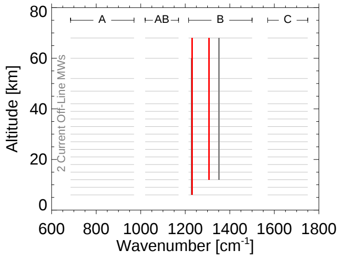
Radiance Contributions at 21km
