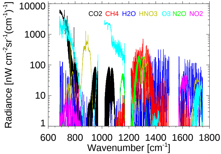
Radiance Contributions at 21km
