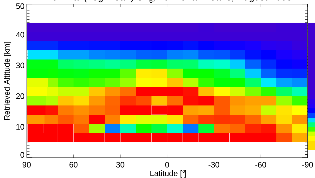
Nominal (Log mean) SF 6 , 10° Zonal Means, August 2003
