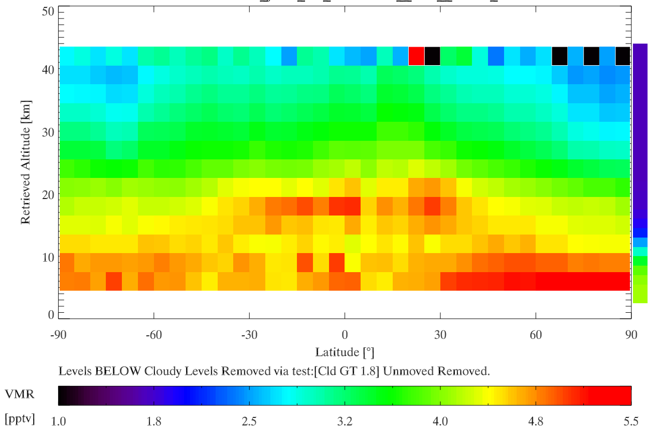
Zonal Mean Jan03MORSE_joint_IG_CorLen50__SF6__04383_04821.050209.sav
