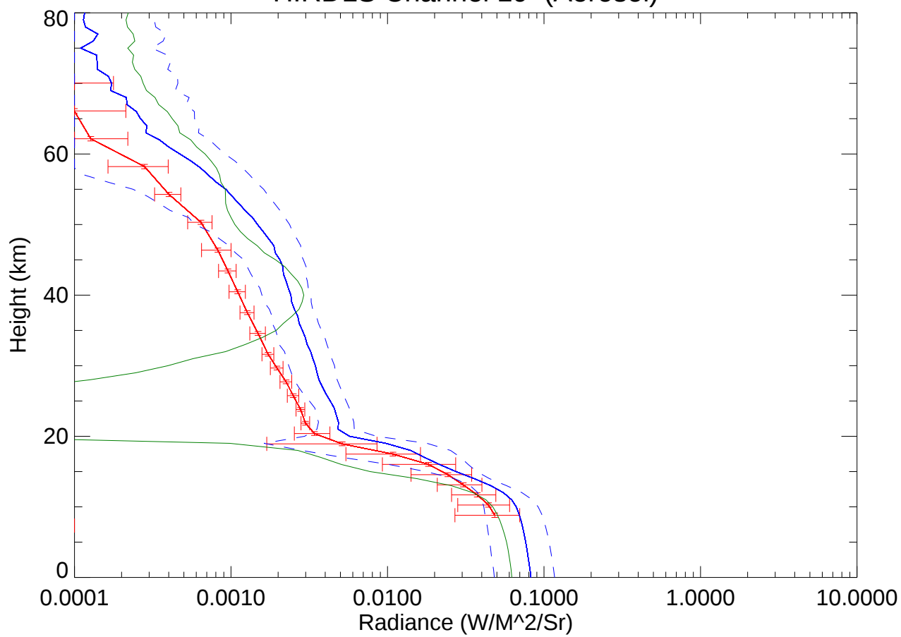
HIRDLS Channel 19 (Aerosol)
