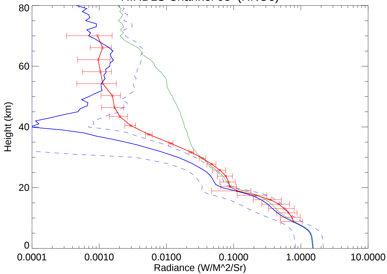
HIRDLS Channel 08 (HNO 3 )
