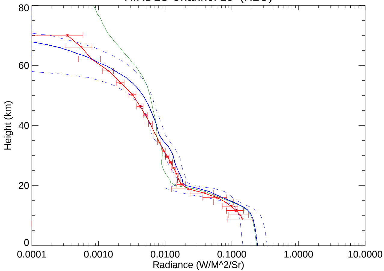
HIRDLS Channel 18 (H2O)
