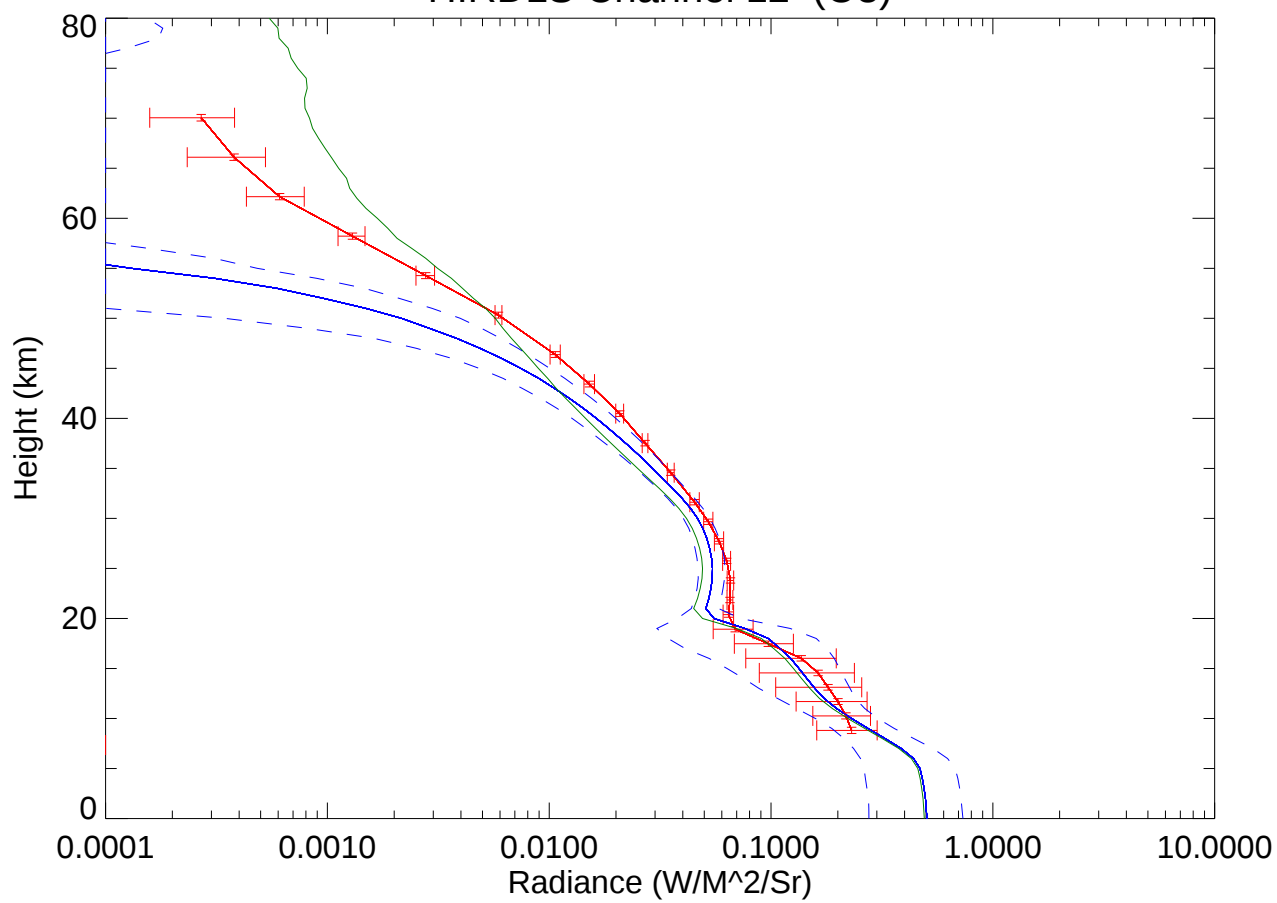
HIRDLS Channel 12 (O3)
