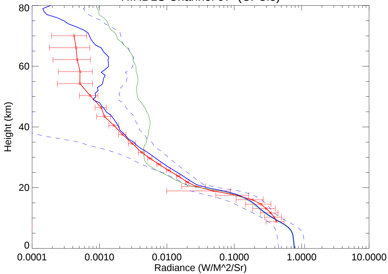
HIRDLS Channel 07 (CFCI3)
