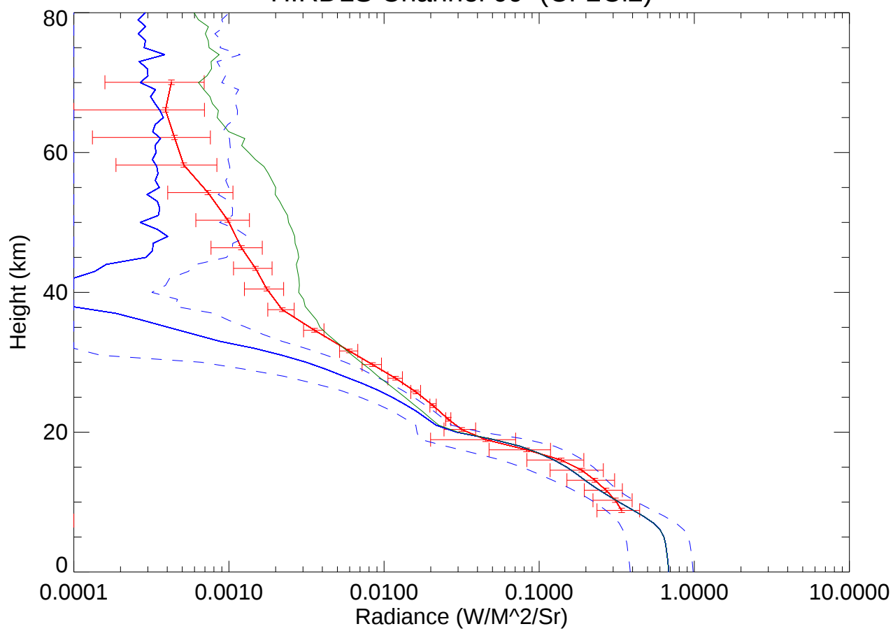
HIRDLS Channel 09 (CF 2 Cl 2 )
