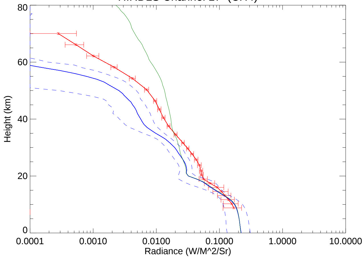
HIRDLS Channel 17 (CH 4 )
