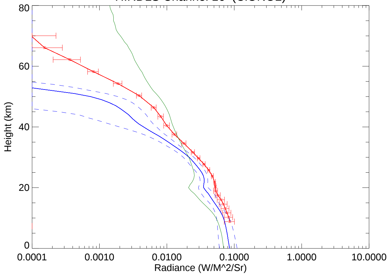
HIRDLS Channel 16 (ClONO2)
