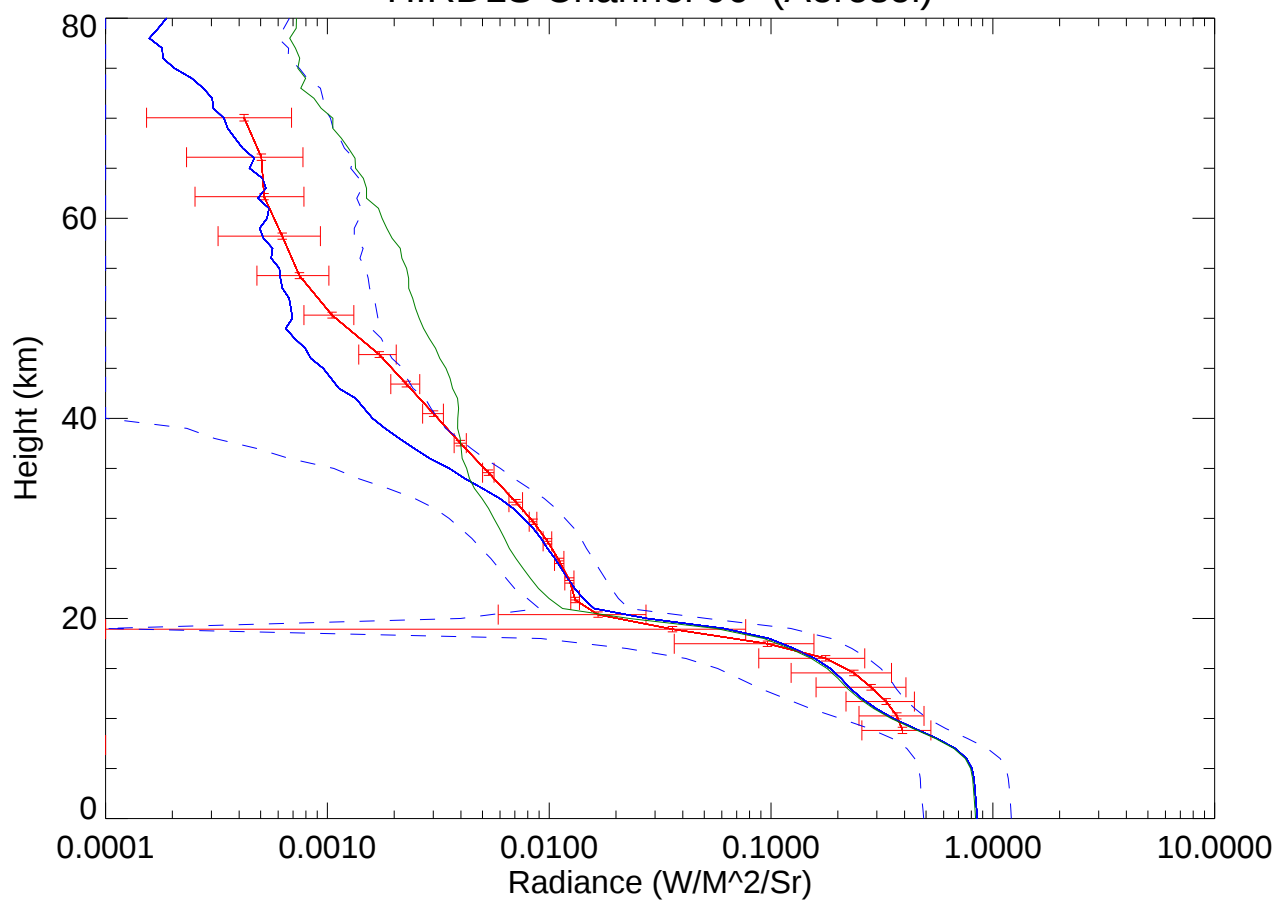
HIRDLS Channel 06 (Aerosol)
