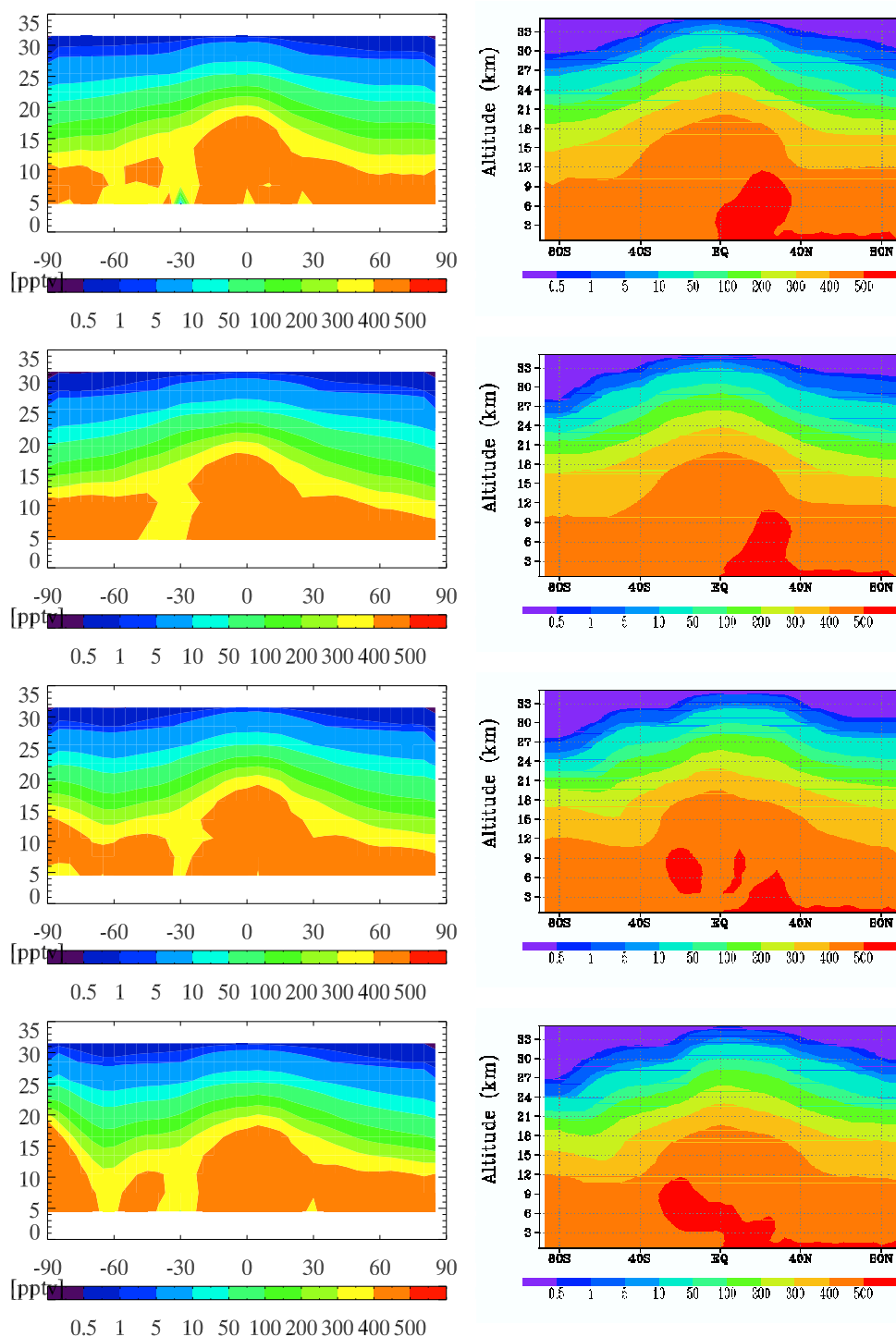
Figure 4.20: Comparison of the equinox and solstice month MIPAS retrieved zonal means with model OCS fields for the same seasons. There is good agreement in general structure. More subtle features, such as the motion of the centre of the tropical tropopause through the year is also visible. [Timmreck. TODO (1)Fix the yellow colour to be inline with her colourscale... (2)Need to re-run the September month as it suffers from the CO bias!!].
