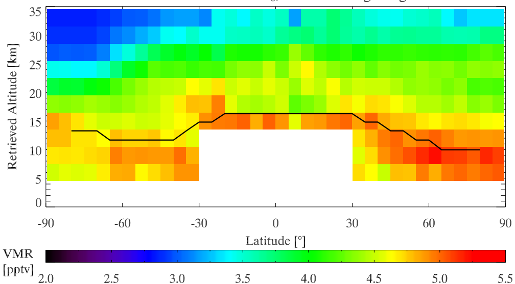
Detrended Zonal Mean SF 6 , after filtering, August 2003
