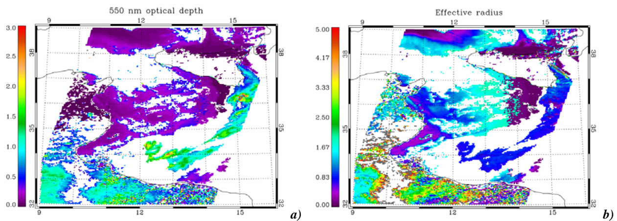
Figure 2. (a) AATSR derived AOT map; (b) AATSR derived particle effective radius.
