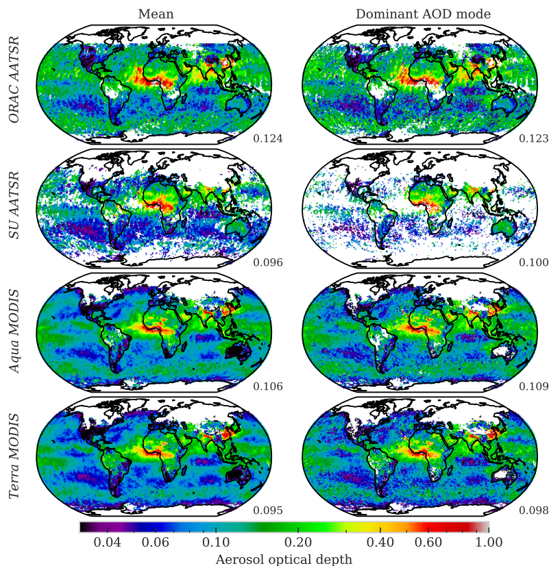
Average aerosol optical depth in January 2008 observed by four satellite records (rows), contrasting a simple mean (left) with the most common mode of a statistical fitting (right).
