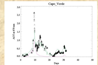
Figure 9: Inter-comparison between AERONET data (white triangles) from the Cape Verde site in the Cape Verde Islands (22.94°N, 16.73°N) and the corresponding model and assimilated model optical depth at 870 nm (pink and green lines). AERONET data courtesy of NASA (PI of the site is Didier Tanré).
