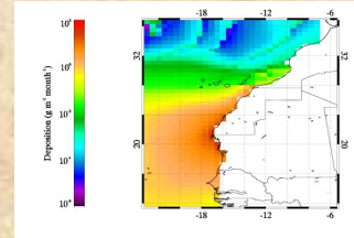
Figure 7- Dust deposition into the Atlantic, March 2006. The total was 3.4 Tg.
