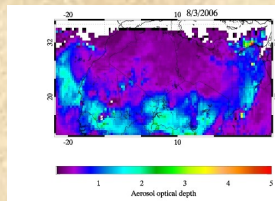
Figure 8: DRI AOD at 550 nm (using data provided by Elisa Carboni, private communication) on 8/3/2006.
