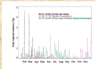
Figure 4: Time-series of emissions from 3 source regions in the Sahara, 2006.
